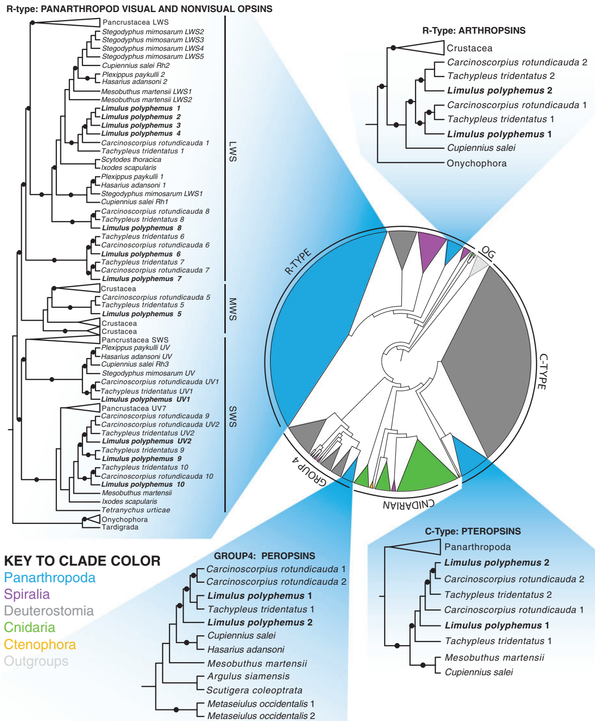
FIG. 2. —Opsin phylogeny. Maximum-likelihood tree of 743 genomic and expressed opsin sequences illustrating the four major evolutionary clades of opsins (C-type, R-type, Cnidarian, and Group 4), divided into subclades by major taxonomic groups (see key for color codes). Panarthropod groups are expanded to highlight the relationships among Limulus polyphemus (in bold) and arachnid and other xiphosuran opsin sequences. For the R-type clade containing the known panarthropod opsin genes, the spectral clades have been indicated as long wavelength sensitive (LWS), middle wavelength sensitive (MWS), and short wavelength sensitive (SWS). Black circles on branches indicate nodal support >80%.
