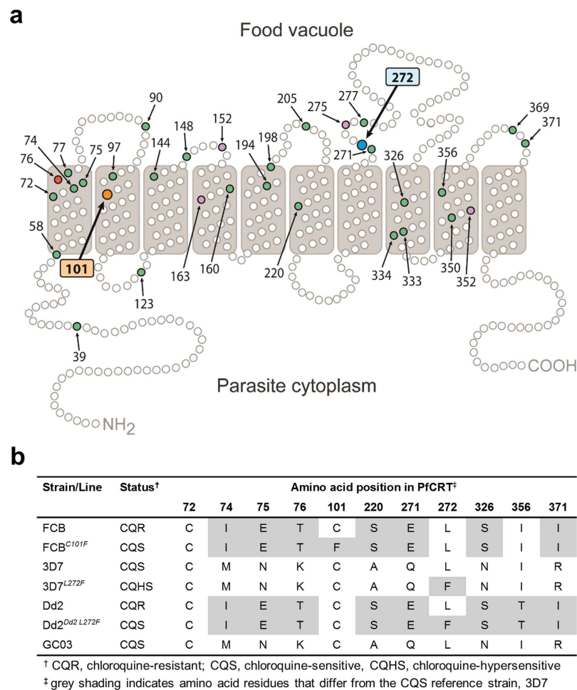
Figure 1. PfCRT mutations. (a) Schematic representation of PfCRT and positions of previously identified polymorphisms 8,71 from field isolates (green circles) and from drug-pressed laboratory lines (purple circles). The critical CQ resistance mutation site (K76) is shaded red, and the two residues at which mutations are described in this study are shaded in orange (C101) and blue (L272). (b) PfCRT haplotypes included this study.
