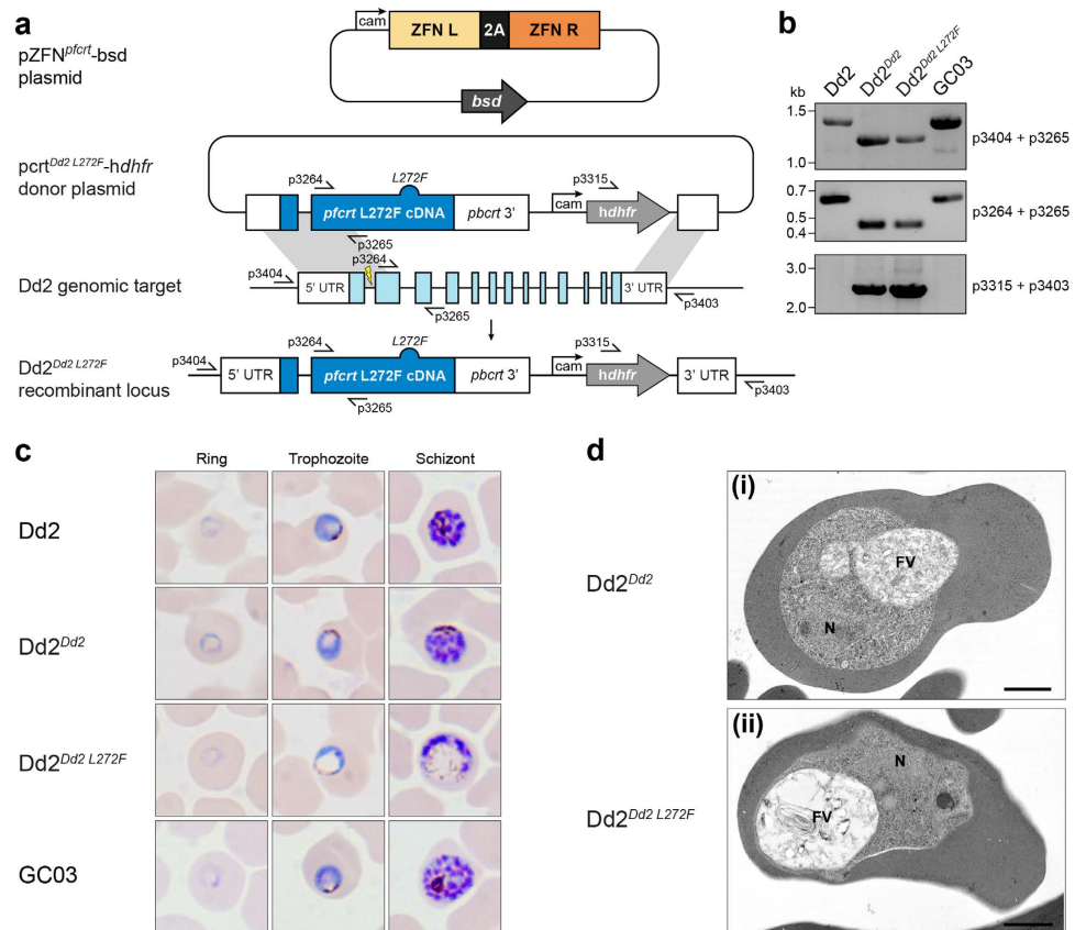
Figure 4. Introduction of PfCRT L272F into Dd2. (a) Schematic of zinc-finger nuclease (ZFN)-mediated generation of vacuole-enlarged parasites. Dd2 parasites were first enriched for the episomal p crT Dd2 L272F-hdhfr or p crT Dd2 -hdhfr donor plasmids (latter not shown). The donor plasmids encoded a cDNA copy of the Dd2 pfcrT allele (dark blue, plasmid), either L272F-mutated (dark blue bump) or wild-type (not shown), followed by a dhfr selection cassette (light grey). Each donor-enriched parasite was then transfected with the pZFN pfcrL -bsd plasmid, expressing the genomic (light blue) pfcrT intron 1-targeting ZFN pair (ZFN L and ZFN R, orange) and the bsd selection cassette (dark grey). ZFN-induced recombination in pfcrT yielded either control Dd2 Dd2 (not shown) or Dd2 Dd2 L272F parasites (dark blue, locus). (b) PCR verification of parental, recombinant control, and Dd2 Dd2 L272F parasite clones. Primer (p) positions are shown in panel a. (c) Light microscope analysis of representative examples of parental, recombinant control, and experimental parasite clones. Ring morphology for each parasite Dd2, Dd2 Dd2 , Dd2 Dd2 L272F, and GC03 was normal. Progression through the trophozoite and schizont stages showed normal morphological development except for the Dd2 Dd2 L272F clone, which exhibited the characteristic enlarged vacuole and diffuse hemozoin phenotypes seen in 3D7 L272F and FCB C101F Giemsa stained parasites. (d) Transmission electron micrographs of Dd2 Dd2 (i) and Dd2 Dd2 L272F parasites (ii) showing similar cytoplasmic appearances except for the enlarged food vacuole (FV) in Dd2 Dd2 L272F. Note neither parasite exhibits knobs. This confirms similar morphological appearances to those of 3D7 and 3D7 L272F , respectively but without knob formation. N—Nucleus. Bars represent 1 μm.
